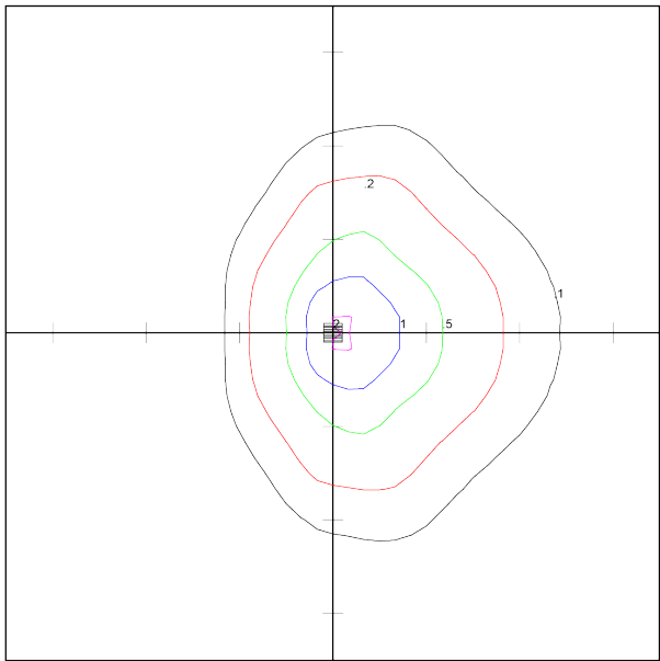
Tamlite Lighting Canada TLMP155K-120-BZ-PC 155W LED MINI WALL PACK WITH PHOTO CELL Horizontal Footcandles Scale: 1 Inch = 10 Ft. Light Loss Factor = 1.00 Lumens Per Lamp = N.A. (absolute photometry) Luminaire Lumens = 986 Mounting Height = 10.00 Ft. Maximum Calculated Value = 2.03 Fc Arrangement: Single
