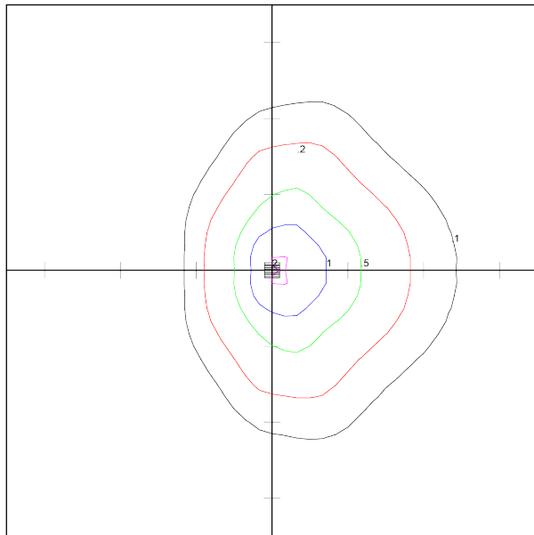
TamLite Lighting Canada TLMWP14LED/PC 14W LED MINI WALL PACK WITH PHOTO CELL Horizontal Footcandles Scale: 1 Inch = 10 Ft Light Loss Factor = 1.00 Lumens Per Lamp = N.A. (absolute photometry) Luminaire Lumens = 986 Mounting Height = 10.00 Ft Maximum Calculated Value = 2.03 Fc Arrangement: Single
