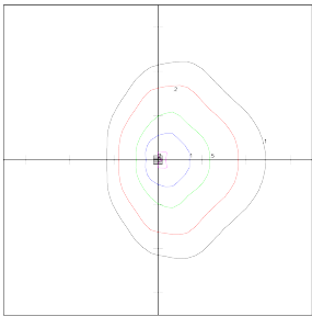
Tamlite Lighting Canada TMWP155K-120-BZ-PC 155W LED MINI WALL PACK WITH PHOTO CELL Horizontal Footcandles Scale: 1 Inch = 10 Ft. Light Loss Factor = 1.00 Lumens Per Lamp = N.A. (absolute photometry) Luminaire Lumens = 986 Mounting Height = 10.00 Ft. Maximum Calculated Value = 2.03 Fc Arrangement: Single
