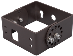
AL-TR-BZ Trunnion Mount Factory prepared 15 degree locking points
